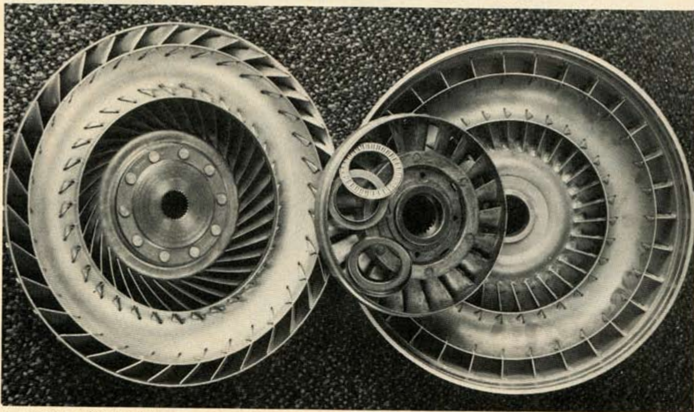
Improved gas mileage and less slippage result from modification of the torque converter. Advanced re-angles the vanes, furnace-brazes the turbines, and adds roller-bearing washers to reduce friction, lower stall speed and improve converter efficiency.
