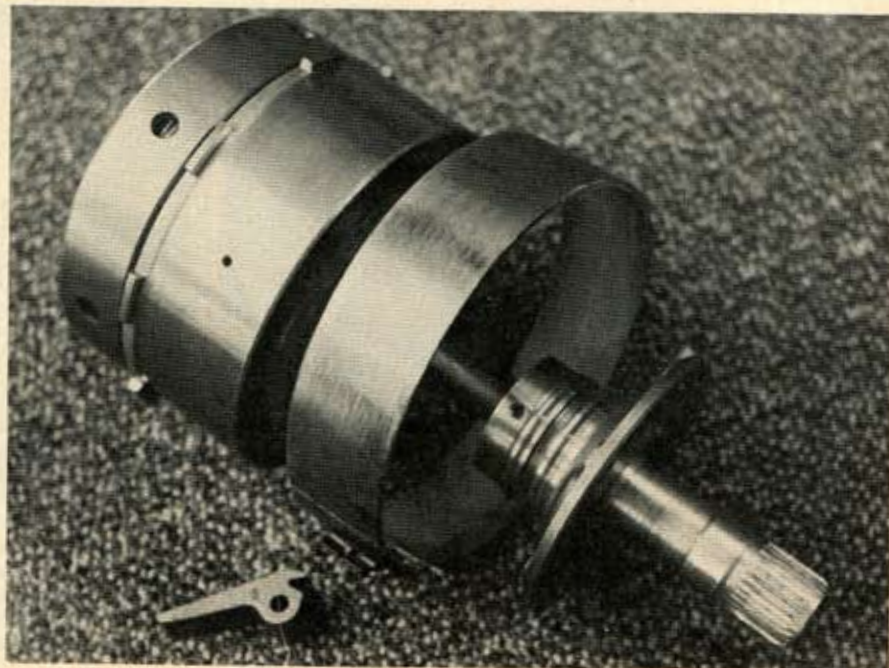
Loosely assembled, the super-duty parts that make the Advanced automatic so tough in MoPar vehicles. Left to right: forward and high gear clutch drums, bands, servo lever with improved ratio tighter shifts and the drilled reaction shaft.
